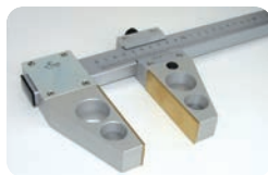
GAUGE FOR LINEAR MEASUREMENTS, WITH LONG JAWS AND STEEL PLATES Page 15.15
