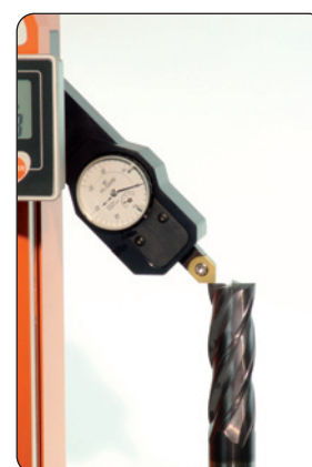
How to measure tool length
